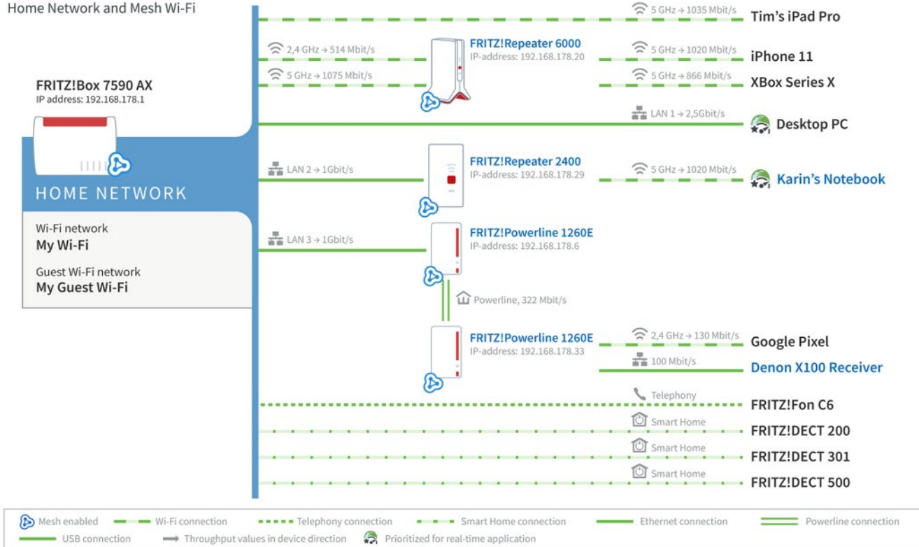
Home Network and Mesh Wi-Fi
